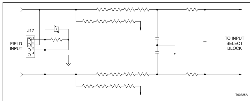
Figure 2-2. Analog Input Circuit
