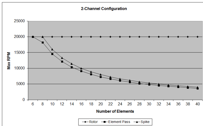
Figure 6: Only One Channel of a Channel Pair is Enabled
